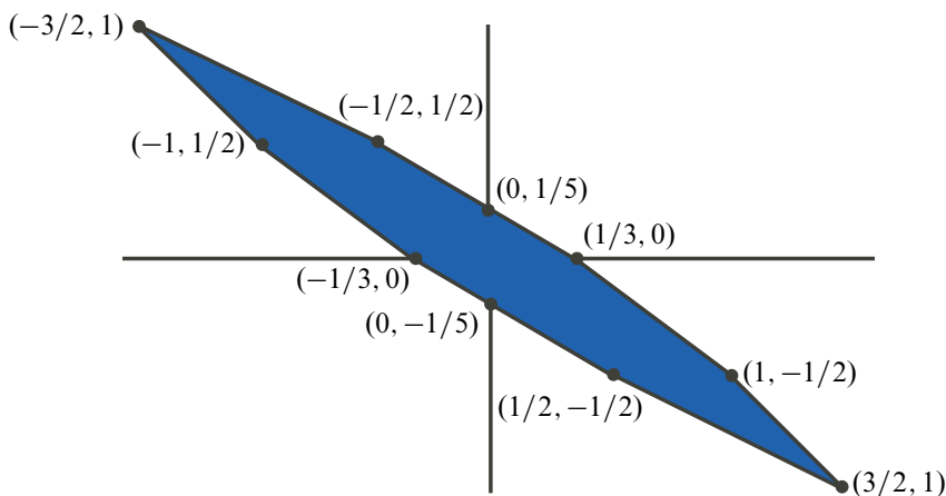
Figure 3: The unit ball for g_{\text{st}} in the span of T_{2,7} and T_{2,11}
