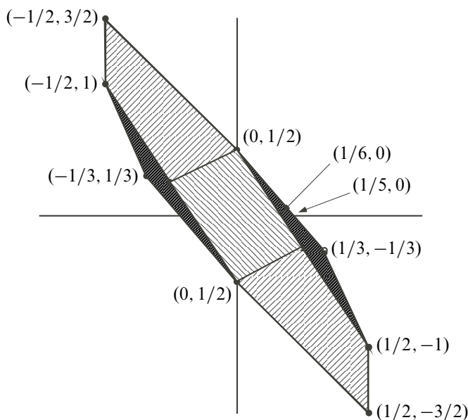
Figure 4: Bounds on the topological and smooth unit ball for g_{\text{st}} on the span \langle T_{3,7} + yT_{2,5} \rangle
